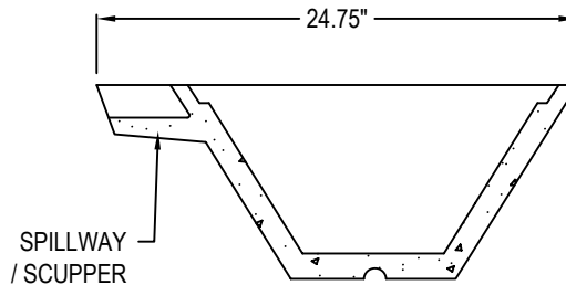
SIDE SECTION
